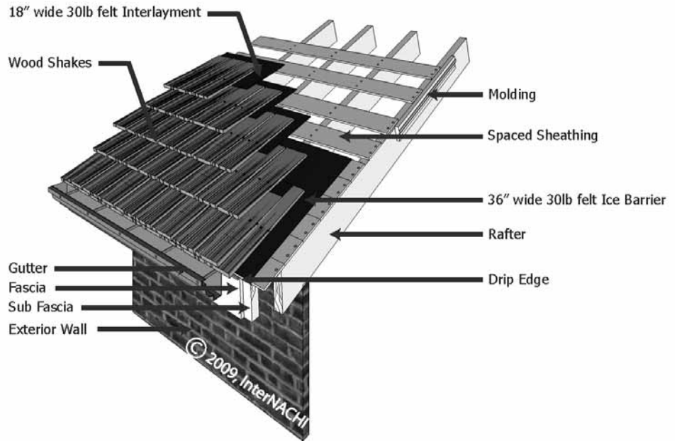
Shakes: Spaced Sheathing
