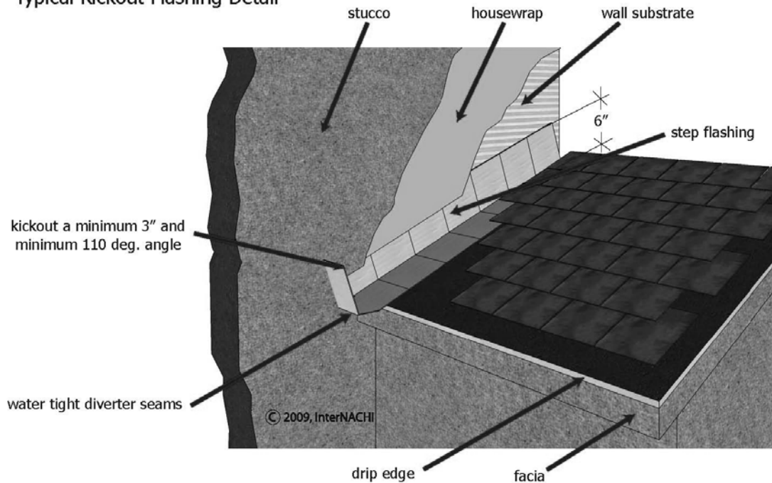
Typical Kickout Flashing Detail
